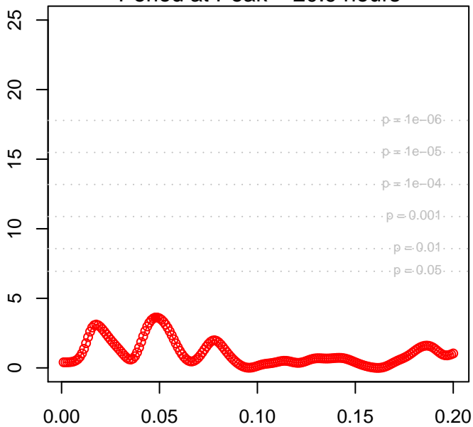
Lomb-Scargle Periodogram Period at Peak = 20.9 hours
