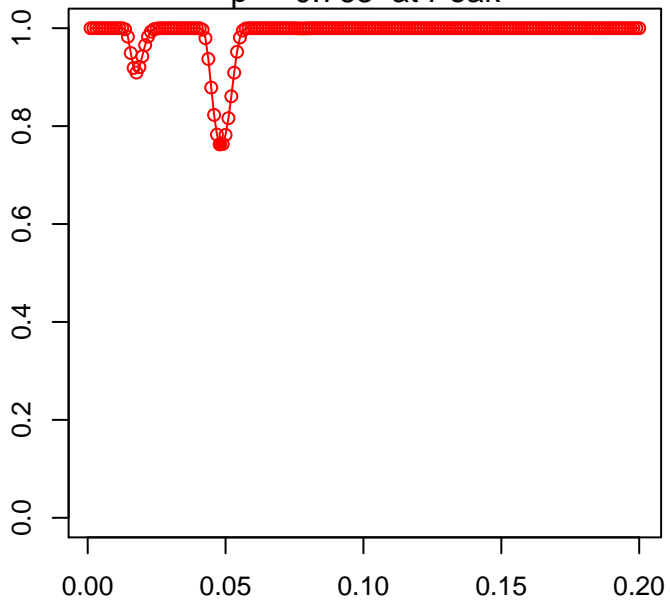
Peak Significance p = 0.763 at Peak
