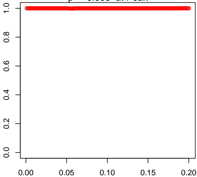
Peak Significance p = 0.998 at Peak
