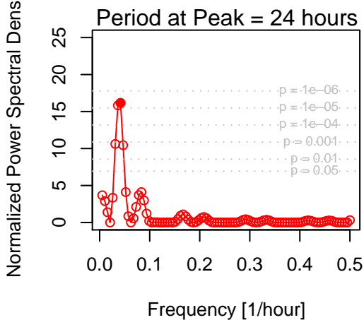
(c) Lomb–Scargle Periodogram
