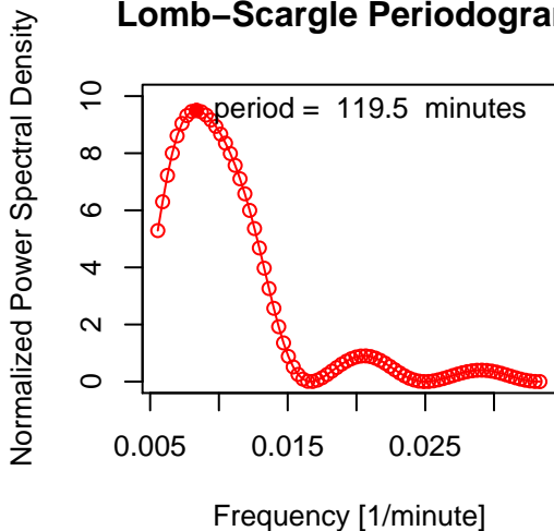
Lomb-Scargle Periodogram
