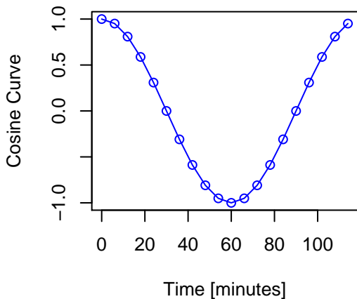
Cosine (N = 20)
