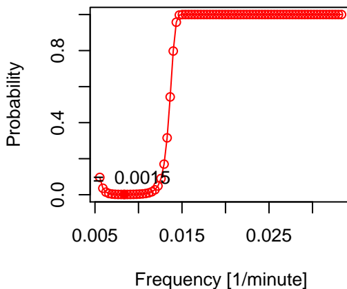
Peak Significance
