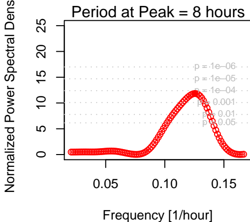
Lomb-Scargle Periodogram
