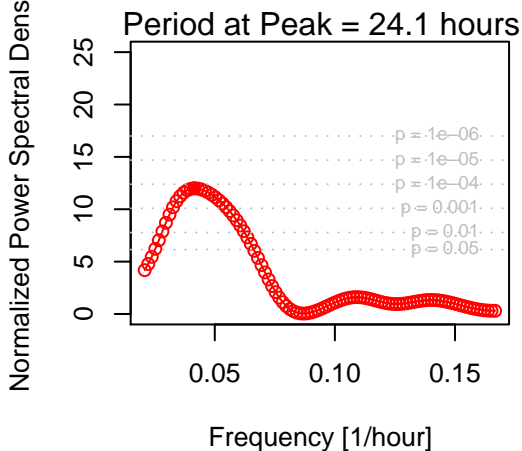
Lomb-Scargle Periodogram
