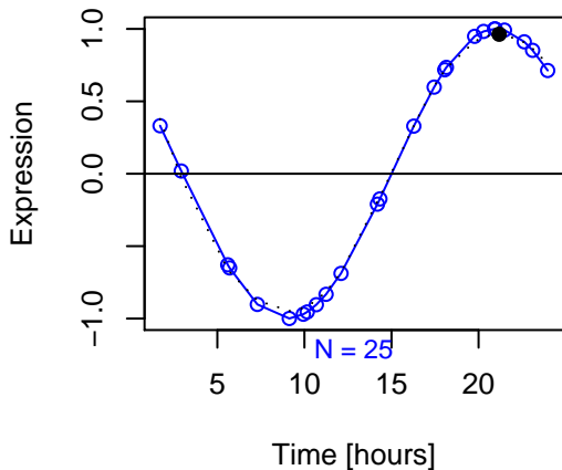
Series5
